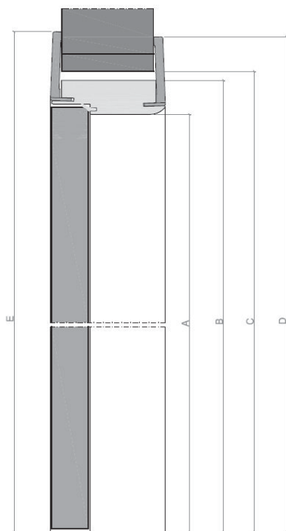
Vertical Section
