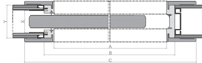
Horizontal Section
